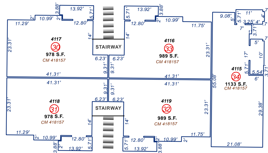
BUILDING 4 FIRST FLOOR
