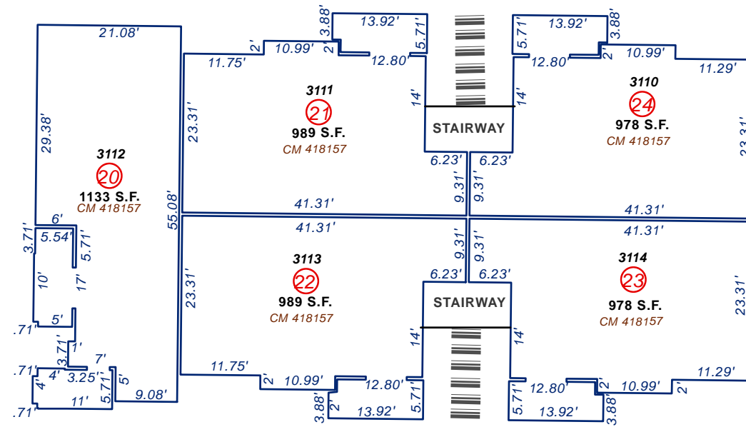
BUILDING 3 FIRST FLOOR
