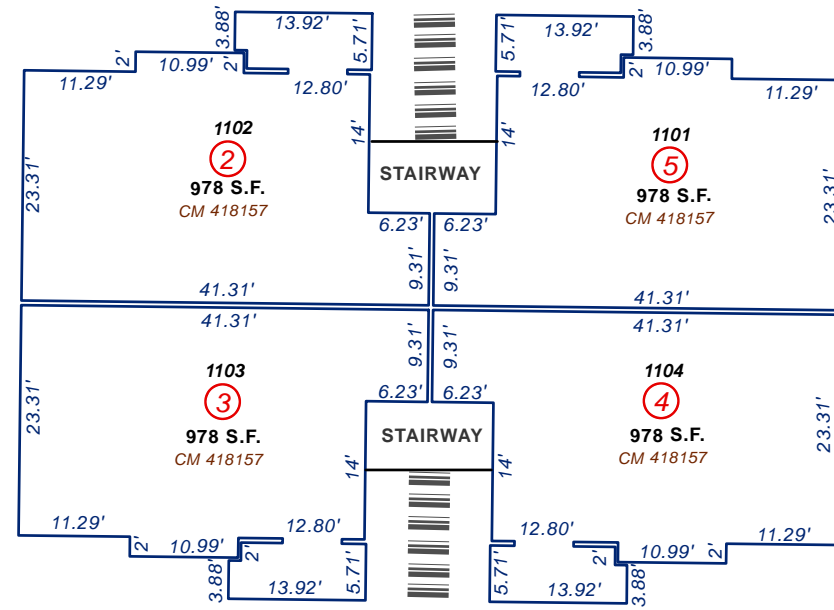
BUILDING 1 FIRST FLOOR
