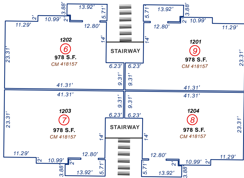
BUILDING 1 SECOND FLOOR
